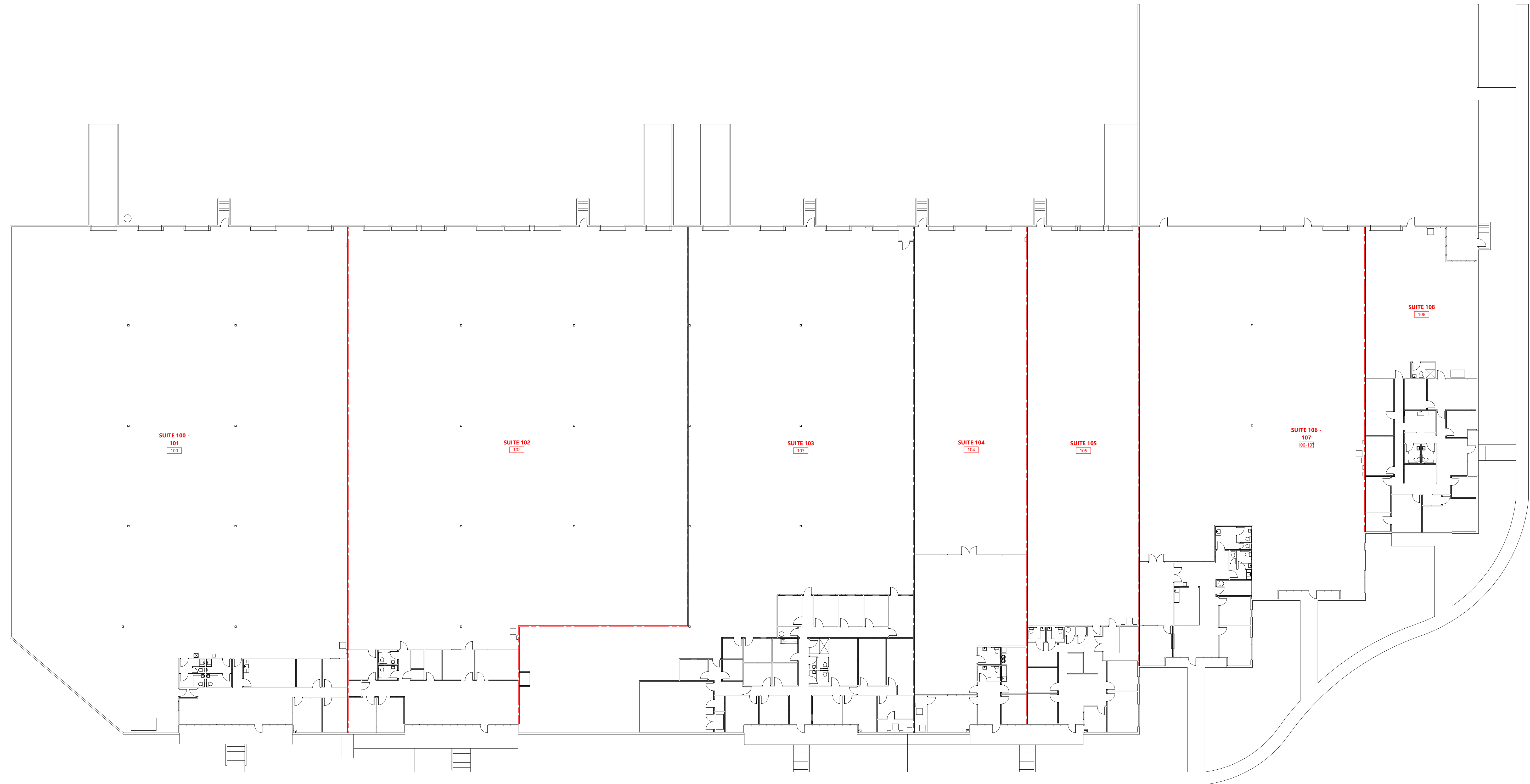
1 FLOOR PLAN - OVERALL 1" = 20'-0"
